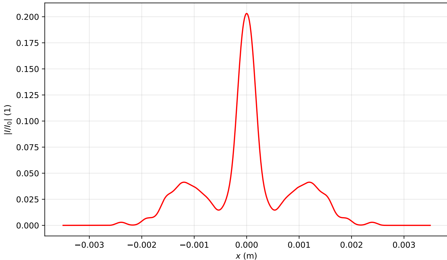
Intensity profile I(x, y = 0, z = 3.105)/I_0 , Pin=8.5Pcr, artificial time
